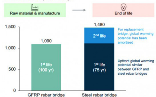
Global warming potential of bridge made with either GFRP or steel, tCO 2 eq over 100 yrs
